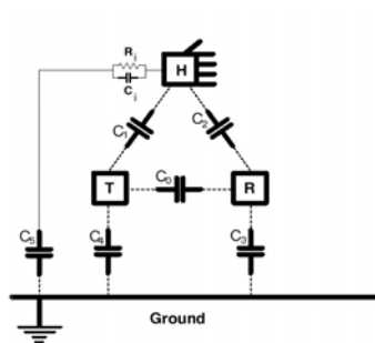
Lumped circuit model of electric field sensing parameters [17].
